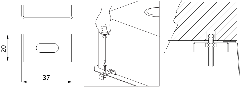
Fixing bracket for undermount sinks
